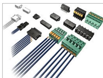
PCB Har-flexicon
